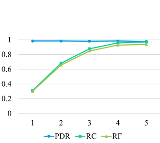
Fig. 6. Evolution of the three metrics across refinement steps.
